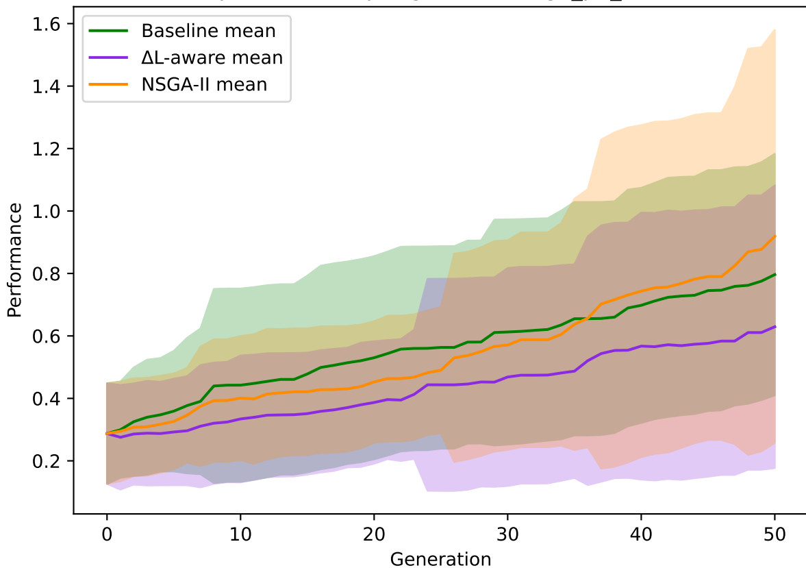
Mean performance per generation (ga_p2_seeds7-7)
