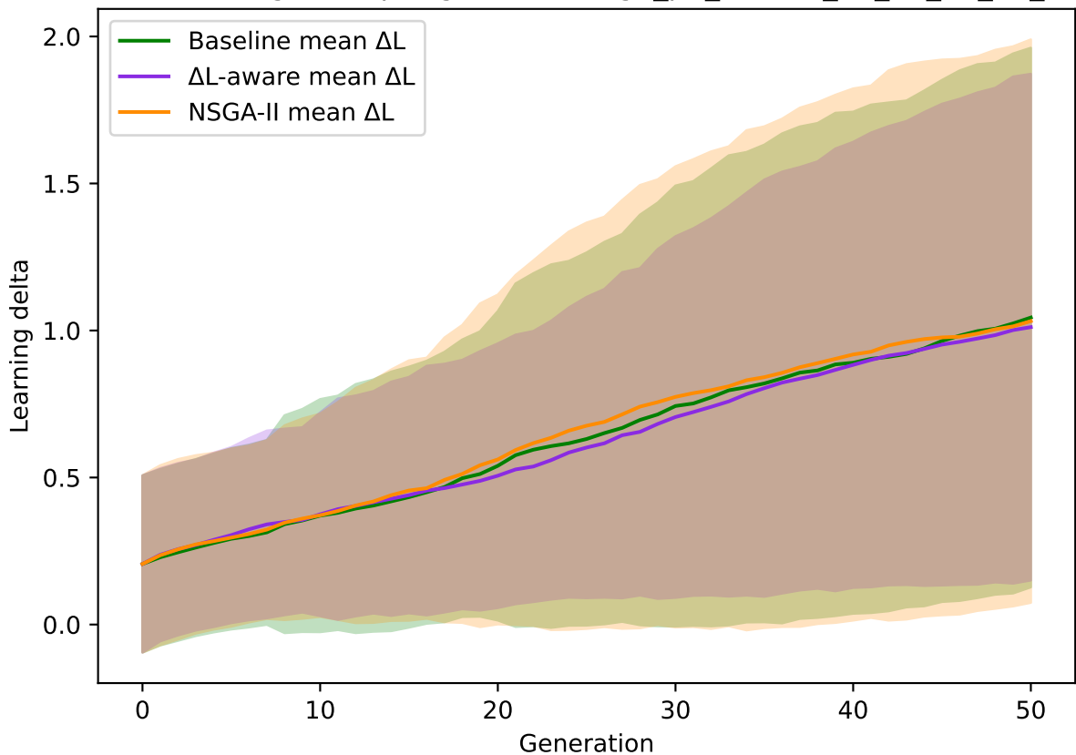
Mean learning delta per generation (ga_p2_seeds7_11_12_13_14_15)
