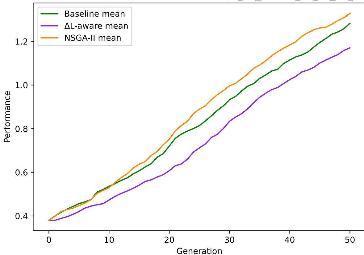
Mean performance per generation, no std (ga_p2_seeds7_11_12_13_14_15)
