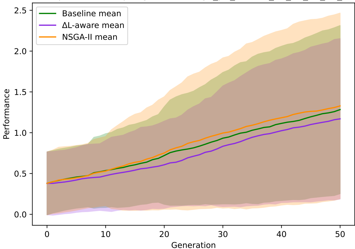
Mean performance per generation (ga_p2_seeds7_11_12_13_14_15)
