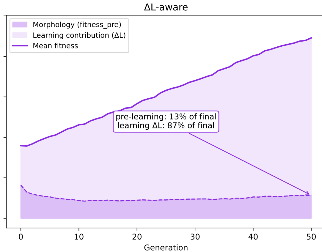
Mean fitness decomposition: morphology vs learning (ga_p2_seeds7_9_10_11_12_13)
