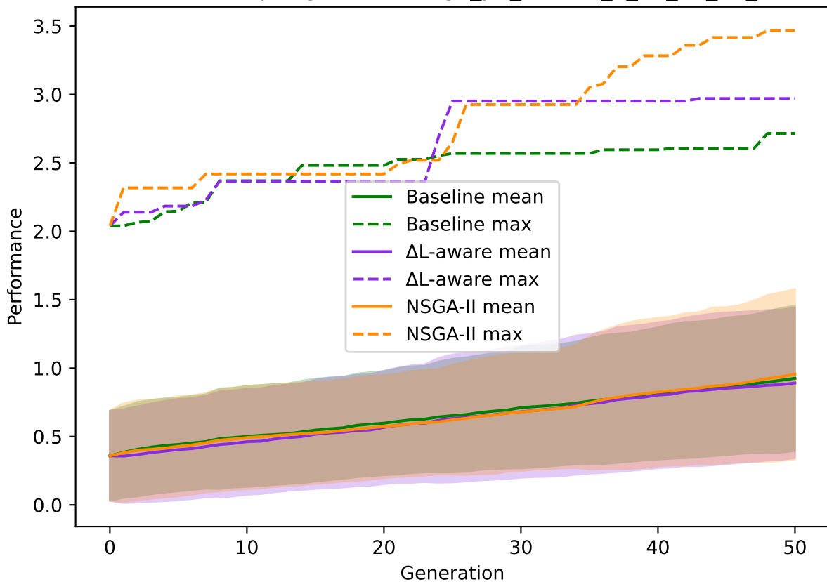
Performance per generation (ga_p2_seeds7_9_10_11_12_13)
