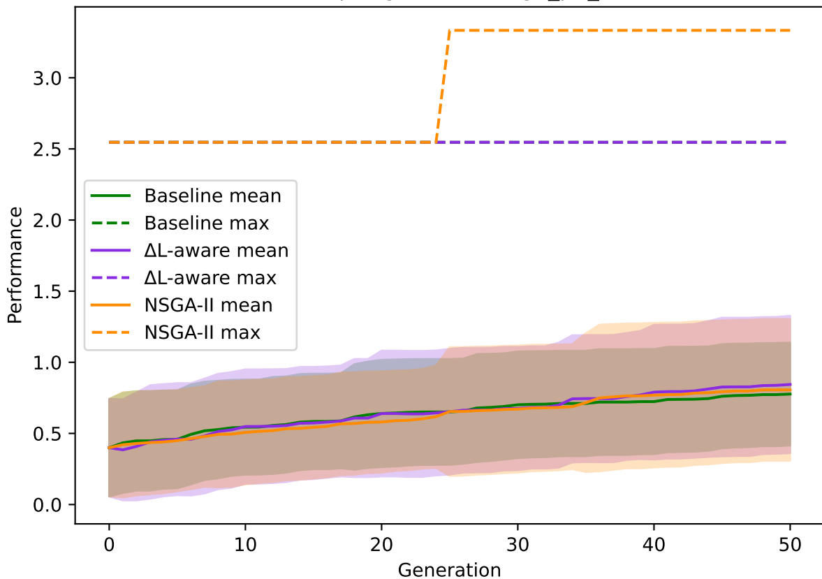
Performance per generation (ga_p2_seeds9-9)
