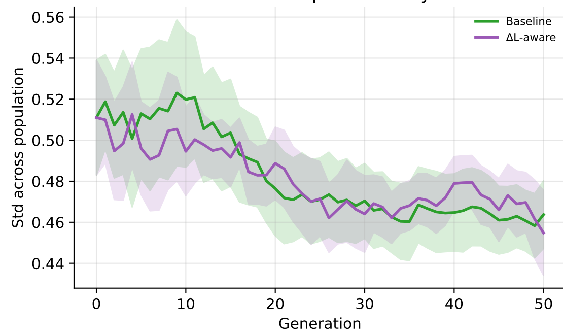
Limb-descriptor diversity
