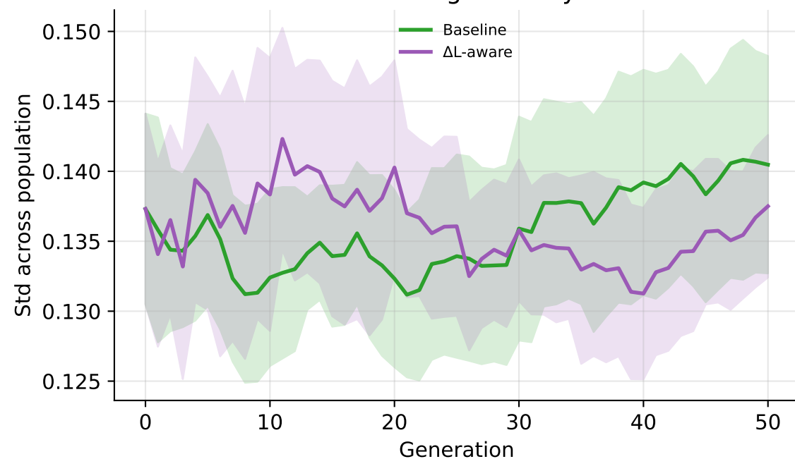
Limb-descriptor diversity
