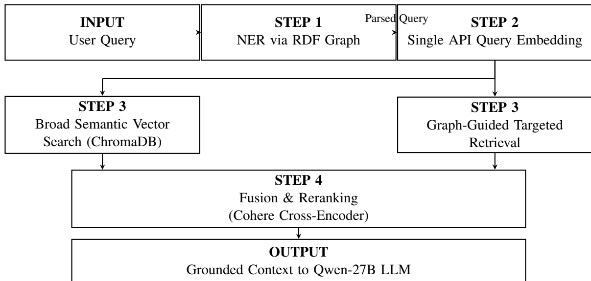
Figure 1: SmartHybridRetriever Pipeline Architecture
