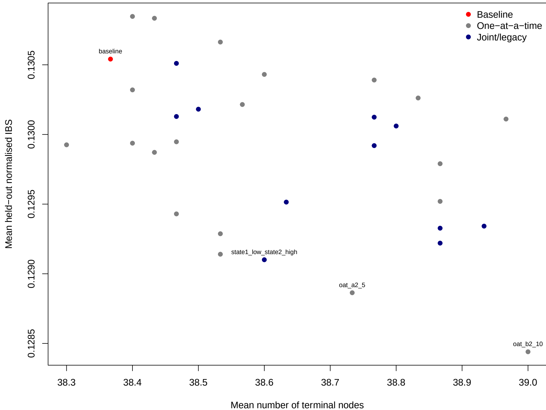
Prediction error versus tree complexity
