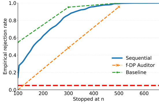
Figure 7: Comparison for \mu_{\text{claim}} = 0.5 (in reality \mu = 1 ) between one-shot t-test (green curve), Algorithm 1 (blue curve) and [5] (orange curve).
