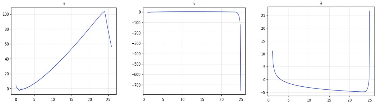
Figure 5: Here we have plotted u, v, \lambda for a target law \nu which is a mixture of the AY and Perkins solutions with weights (\frac{1}{3}, \frac{2}{3}) with \mu \sim \text{Exp}(1) and R given by (12) with \sigma = T = 1 . In this case the AY optimal strike in (4) is K^*(B) = B - 1 and the Perkins optimal strike is K^*(B) = -1 + B - W((Be^B - 1 - e^B)/e) , where W(\cdot) denotes the principal branch of the Lambert- W function, i.e. the unique solution w \geq -1 of we^w = z for z \geq -1/e .
