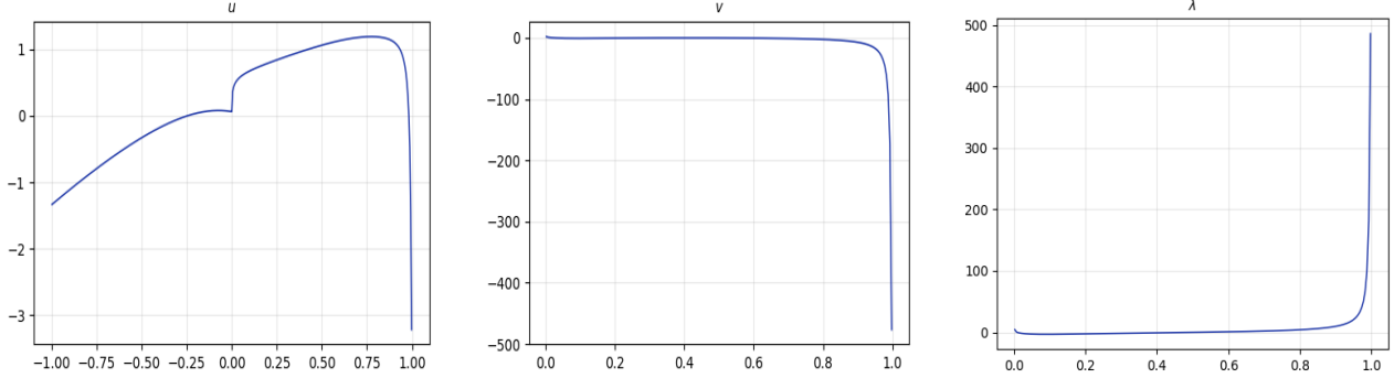
Figure 1: Here we have plotted u, v, \lambda for a target law \nu which is a 60/40 mixture of the Azéma-Yor and Perkins solutions respectively (and hence admissible) with \mu \sim U[-1, 1] , using 400 (equidistant) steps for X direction and 200 for S .
