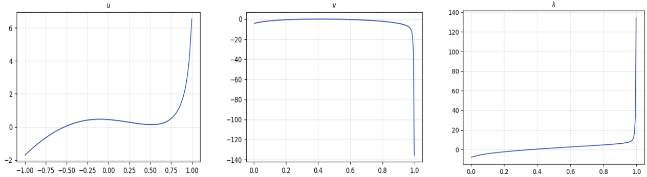
Figure 4: Here we have plotted u , v , \lambda for a target law \nu with cdf \nu([0, s]) = 1 - (1 - s)(1 - \theta s) for s \in [0, 1] (see Example 2.1) with \theta = 1/4 , with all other parameters unchanged.
