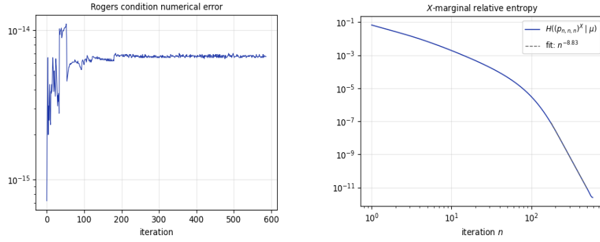
Figure 6: Here we have plotted the error for the Rogers condition for the final \mu \sim \text{Exp}(1) example on the previous page and the (entropic) error for the X -marginal. The log-log slope over iterations 177-498 suggests that H((p_{n,n,n})^X | \mu) \sim Cn^{-8.83} , so the O(\frac{1}{n}) rate reported in Proposition 3.3 may not be sharp (see [CCRW26] for more on this). Code takes about a minute to run on an old MacBook, but we ran to a lower tolerance than is typically necessary in practice.
