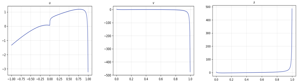
Figure 2: Here we have plotted u , v , \lambda for a target law \nu which is a (\frac{3}{5}, \frac{2}{5}) weighting of the AY and Perkins solutions respectively (so trivially an admissible joint law exists) with \mu \sim U[-1, 1] and R = \mu \otimes \nu , using 400 (equidistant) steps for X direction and 200 for S .
