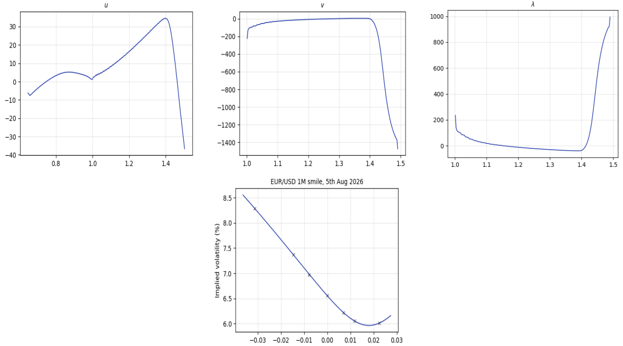
Figure 7: Here we have plotted u , v , \lambda with \mu given by an SVI fit to the EUR-USD smile here ( x -axis is log moneyness in the smile plot, data taken from https://www.investing.com/currencies/eur-usd-options ) with a (made-up) (\frac{1}{3}, \frac{2}{3}) AY-Perkins weighting as above and all other parameters unchanged from the previous plot. The parameters for the SVI fit are (a, b, \sigma, \rho, m) = (0.00016844, 0.00805007, 0.01660353, 0.01493316, 0.01824409) .
