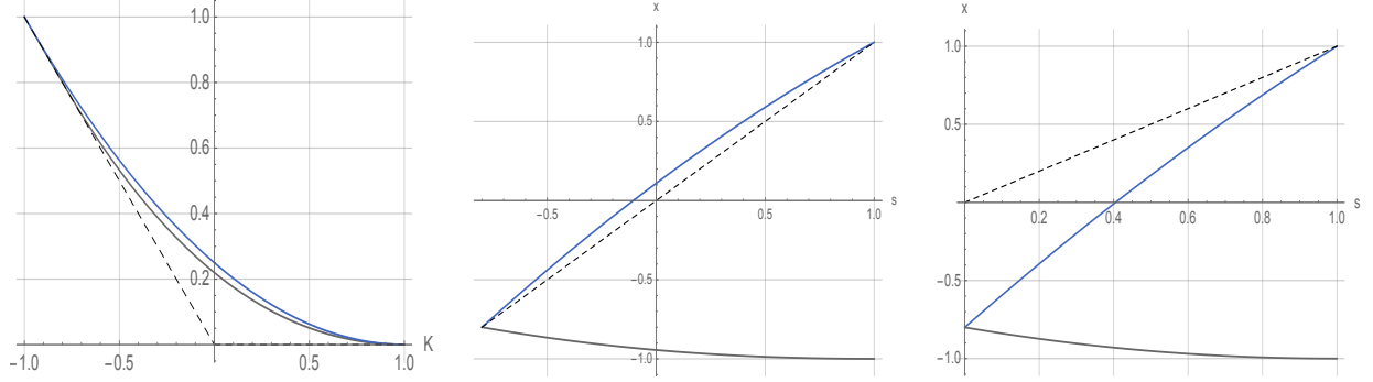
Figure 1: On the left we check the convex order condition for Example 2.1 by pricing call options on Z for a range of strike values K (solid grey) and X (blue), and in the middle we see the upper and lower branches T_u(z) (blue) and T_d(z) (solid grey) for the left curtain coupling, and on the right we see the corresponding x_+(s) (blue) and x_-(s) (solid grey), and we (correctly) see that x_+(s) \leq s .
