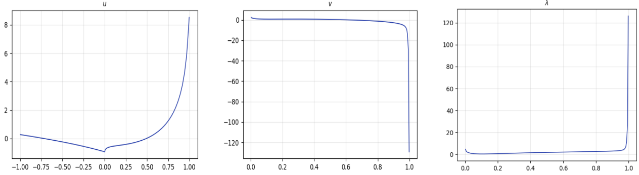
Figure 3: Here we have plotted u , v , \lambda for a target law \nu with cdf \nu([0, s]) = s^p for s \in [0, 1] with p = 3/4 , with all other parameters unchanged.
