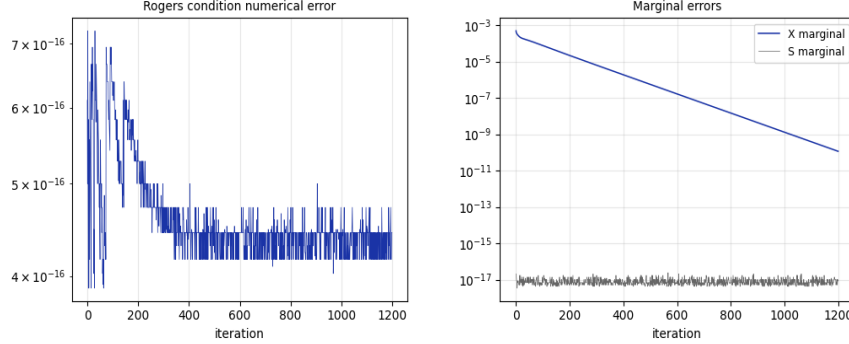
Figure 2: Here we have plotted the error for the Rogers condition and the \mu -marginal condition.
