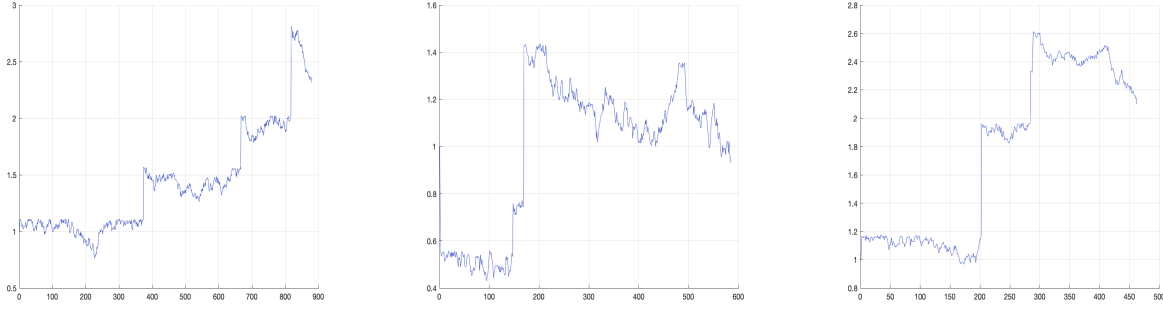
Figure 8: Here we see three simulations of the lost time Rogers Martingale M_t in Section 3.2 with Target laws \mu \sim \text{Exp}(1) and \nu \sim \text{Exp}(1) + \frac{1}{2} , and the AY law here is \text{Exp}(1) + 1 .
