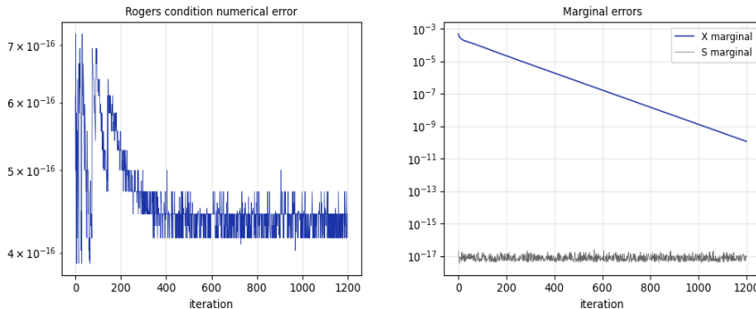
Figure 2: Here we have plotted the error for the Rogers condition and the error for the \mu -marginal condition for the plots above, computed as \max_i |\sum_j P_{ji} - \mu_i| where P_{ji} is the current joint mass on the cell (s_j, x_i) . Code takes about a minute to run on an old MacBook, but we ran to a lower tolerance than is practically necessary here.
