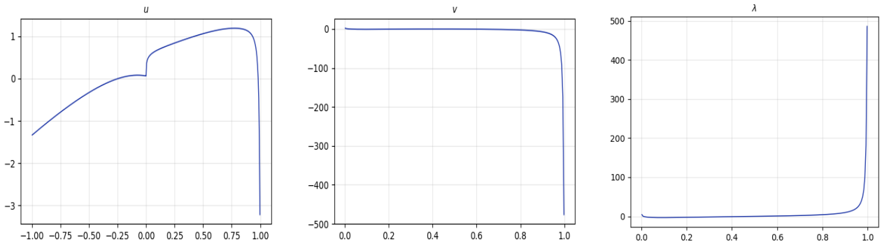
Figure 1: Here we have plotted u , v , \lambda for a target law \nu which is a 60/40 mixture of the Azéma-Yor and Perkins solutions respectively (so trivially an admissible joint law exists) with \mu \sim U[-1, 1] , using 400 (equidistant) steps for X direction and 200 for S .
