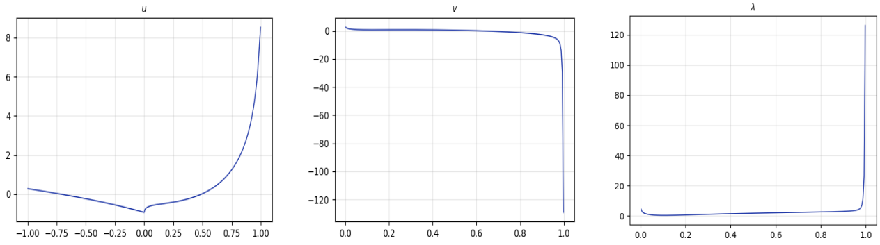
Figure 3: Here we have plotted u , v , \lambda for a target law \nu with cdf \nu([0, s]) = s^p for s \in [0, 1] with p = 3/4 , again with \mu \sim U[-1, 1] .
