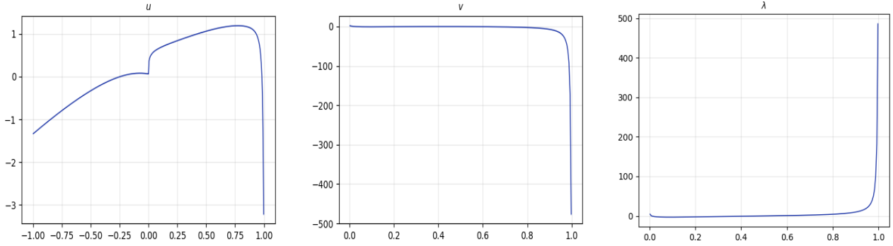
Figure 1: Here we have plotted u, v, \lambda for a target law \nu which is a 60/40 mixture of the Azéma-Yor and Perkins solutions respectively (so trivially an admissible joint law exists) with \mu \sim U[-1, 1] , using 400 (equidistant) steps for X direction and 200 for S .
