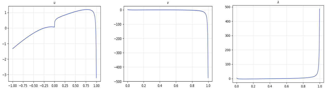
Figure 2: Here we have plotted u , v , \lambda for a target law \nu which is a 60/40 mixture of the Azéma-Yor and Perkins solutions respectively (so trivially an admissible joint law exists) with \mu \sim U[-1, 1] and R = \mu \otimes \nu , using 400 (equidistant) steps for X direction and 200 for S .
