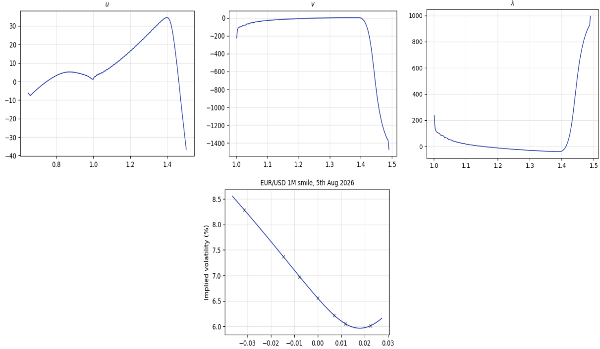
Figure 7: Here we have plotted u , v , \lambda with \mu given by an SVI fit to the EUR-USD smile here ( x -axis is log moneyness in the smile plot, data taken from https://www.investing.com/currencies/eur-usd-options ) with a (\frac{1}{3}, \frac{2}{3}) weighting and all other parameters unchanged from the previous plot. The SVI parameters are (a, b, \sigma, \rho, m) = (0.00016844, 0.00805007, 0.01660353, 0.01493316, 0.01824409) .
