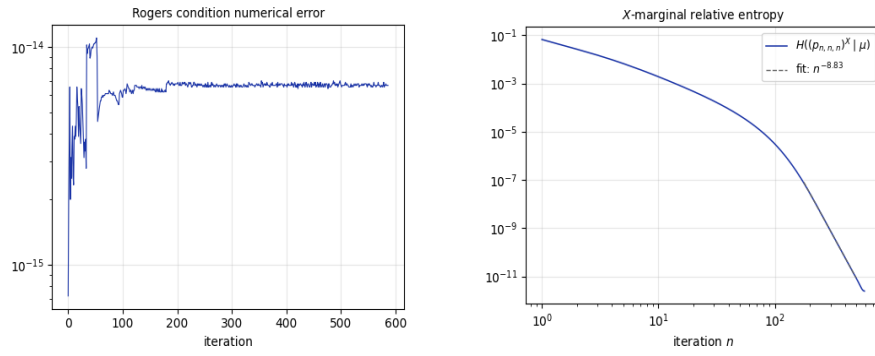
Figure 6: Here we have plotted the error for the Rogers condition for the final \mu \sim \text{Exp}(1) example on the previous page and the error for the X . The log-log slope over iterations 177-498 suggests that H((p_{n,n,n})^X | \mu) \sim Cn^{-8.83} , so the linear convergence rate reported in Proposition 3.3 may not be sharp (see [CCRW26] for more on this). Code takes about a minute to run on an old MacBook, but we ran to a lower tolerance than is practically necessary here.
