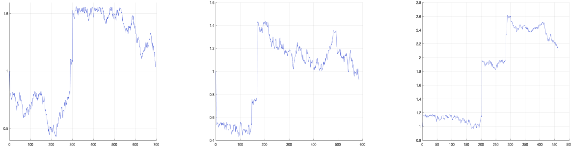
Figure 8: Here we see three simulations of the lost time Rogers Martingale M_t in Section 3.2 with Target laws \mu \sim \text{Exp}(1) and \nu \sim \text{Exp}(1) + \frac{1}{2} , and the AY law here is \text{Exp}(1) + 1 .
