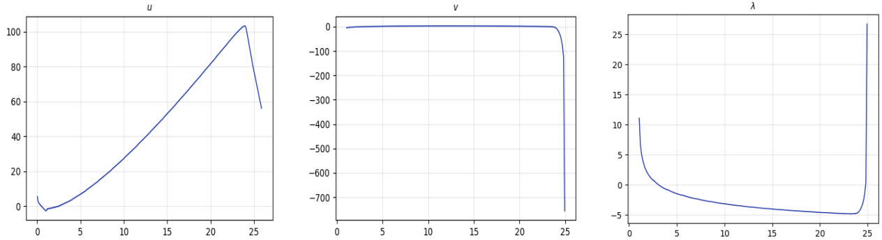
Figure 5: Here we have plotted u , v , \lambda for a target law \nu which is a (\frac{1}{3}, \frac{2}{3}) weighting of AY and Perkins with \mu \sim \text{Exp}(1) and R given by (12) with \sigma = T = 1 . In this case the AY optimal strike in (4) is K^*(B) = B - 1 and the Perkins optimal strike is K^*(B) = -1 + B - W((Be^B - 1 - e^B)/e) , where W(\cdot) denotes the principal branch of the Lambert- W function, i.e. the unique solution w \geq -1 of we^w = z for z \geq -1/e .
