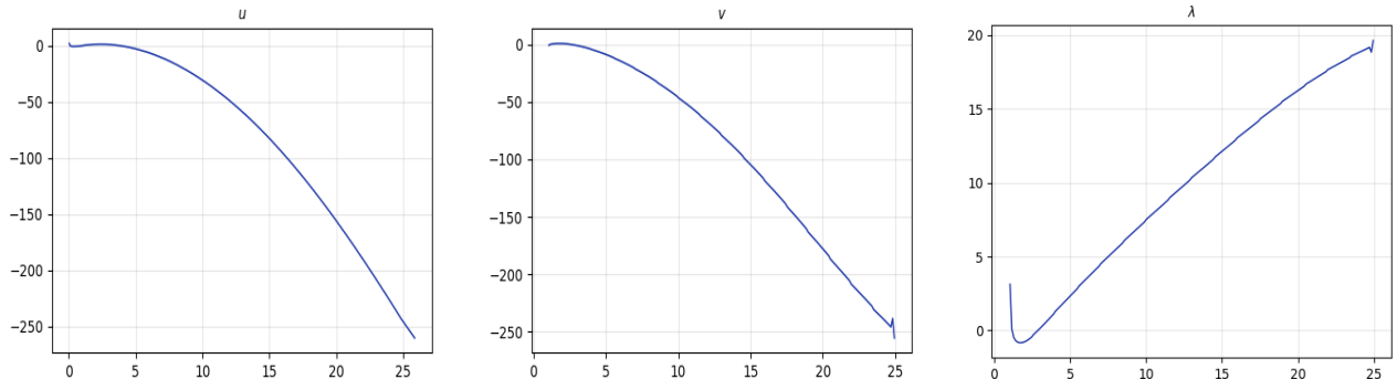
Figure 6: Here we have plotted u , v , \lambda for a target law \nu which is a mixture of the AY and Perkins solutions with weights (\frac{2}{3}, \frac{1}{3}) with \mu \sim \text{Exp}(1) and R given by (12) with \sigma = T = 1 . In this case the Perkins optimal strike in (4) is K^*(B) = -1 + B - W((Be^B - 1 - e^B)/e) , where W(\cdot) denotes the principal branch of the Lambert- W function, i.e. the unique solution w \geq -1 of w e^w = z for z \geq -1/e ; the argument above is \geq -1/e exactly when B \geq 1 , so K^*(B) is real for all barriers above X_0 = 1 , and the AY optimal K^*(B) = B - 1 .
