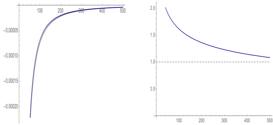
Figure 4: Here we have plotted the numerical solution to the VIE (22) using an Adams scheme (grey) verses the linearized approximation \hat{\psi}^\infty (blue) for \nu = .25 , \lambda = 1 and H = .25 , and in the second graph we have plotted the ratio of these two terms.
