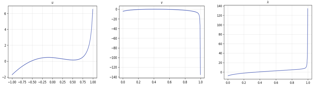
Figure 4: Here we have plotted u , v , \lambda for a target law \nu with cdf \nu([0, s]) = 1 - (1 - s)(1 - \theta s) for s \in [0, 1] (see Example 2.1) with \theta = 1/4 , again with \mu \sim U[-1, 1] .
