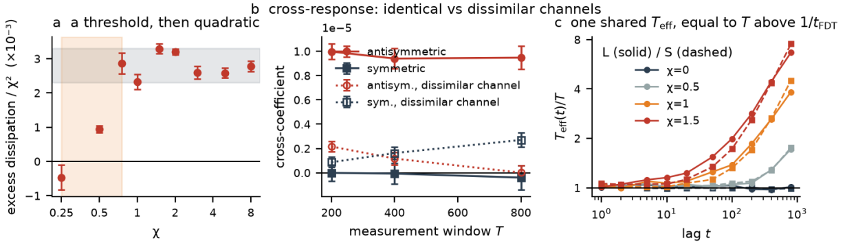
FIG. 4. Dissipation and response. (a) Excess dissipation per particle against \chi , each point probed from a configuration equilibrated at that \chi , with the quadratic form. (b) Symmetric and antisymmetric parts of the differential cross-response between two nonreciprocal channels, against measurement window. For channels of identical structure the symmetric part is consistent with zero at every window while the antisymmetric part is stable; the structurally dissimilar control is plotted alongside on the same axes, where the pattern inverts. (c) Effective temperature against measurement window: flat at \chi = 0 , where it calibrates to k_B T , and growing as t^{0.89} at \chi = 1.5 with no plateau. Inset: mean-squared displacement of the system centre of mass, near-ballistic at \chi = 1.5 over these windows ( t^{1.96} ) and diffusive at \chi = 0 ( t^{1.01} ).
