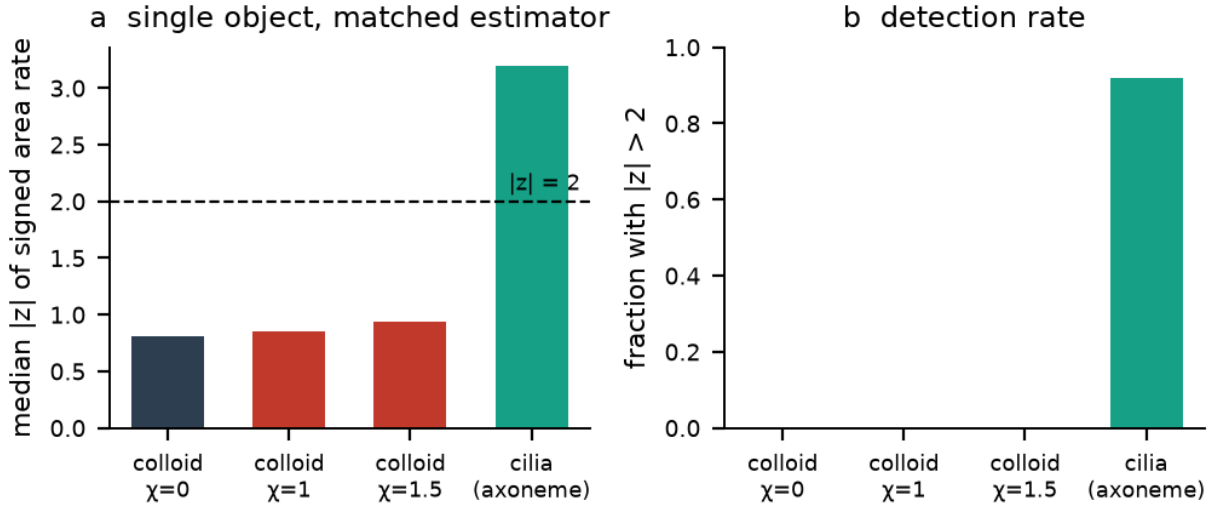
FIG. 5. Circulation at matched level of description. (a) Median |z| of the signed area rate for a single tracked colloidal cluster at three values of \chi , against a single Chlamydomonas axoneme, using the identical estimator, shape-descriptor reduction to two modes, and phase-randomised surrogate protocol. (b) The fraction of objects exceeding |z| = 2 . No circulation is detectable in the tracked colloidal clusters; axonemes show it in 92% of cases.
