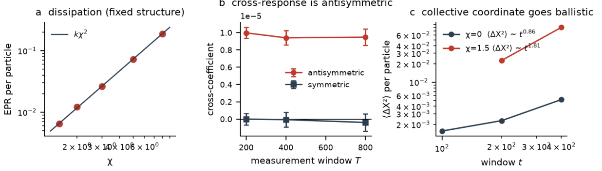
FIG. 5. Dissipation and response. (a) Excess dissipation per particle against \chi , each point probed from a configuration equilibrated at that \chi , with the quadratic form. (b) Symmetric and antisymmetric parts of the differential cross-response between two nonreciprocal channels, against measurement window. For channels of identical structure the symmetric part is consistent with zero at every window while the antisymmetric part is stable; the structurally dissimilar control is plotted alongside on the same axes, where the pattern inverts. (c) Effective temperature against measurement window: flat at \chi = 0 , where it calibrates to k_B T , and growing as t^{0.89} at \chi = 1.5 with no plateau. Inset: mean-squared displacement of the system centre of mass, near-ballistic at \chi = 1.5 over these windows ( t^{1.96} ) and diffusive at \chi = 0 ( t^{1.01} ).
