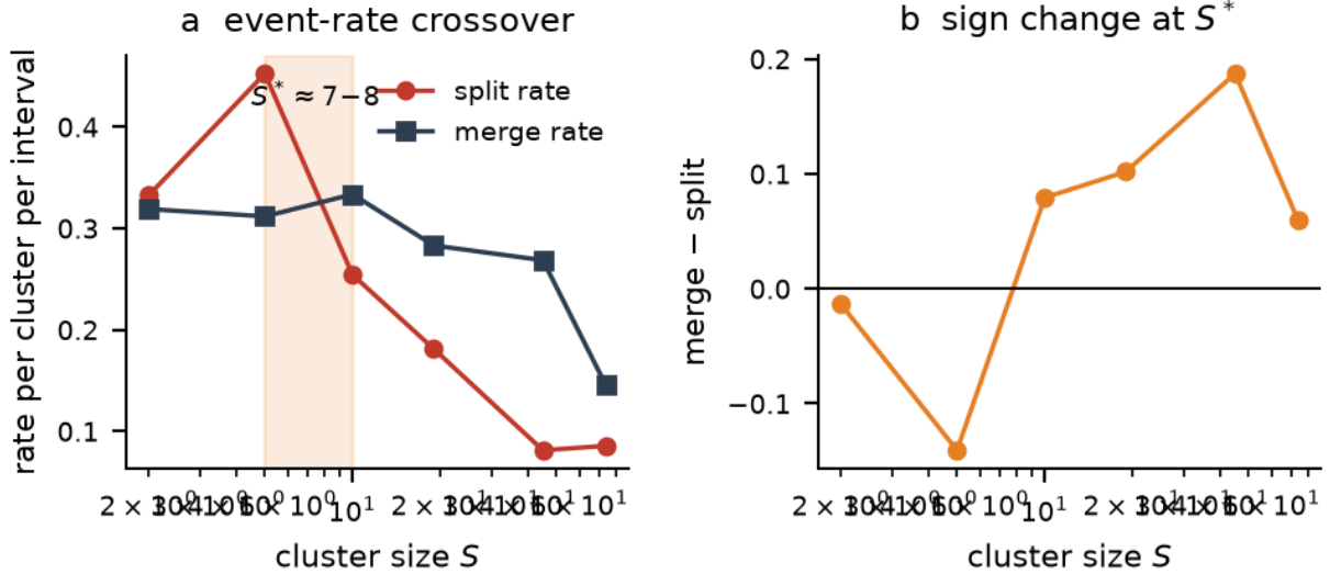
FIG. 4. The event-rate crossover. (a) Per-cluster split and merge rates against cluster size, measured at \Delta t = 50 from equilibrated configurations (105,708 cluster observations). The rates cross between the size-5 and size-10 bins. (b) Their difference, showing the sign change. Splitting dominates below the crossing, merging above it.
