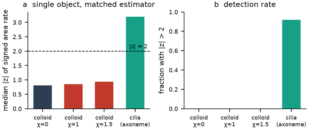
FIG. 6. Circulation at matched level of description. (a) Median |z| of the signed area rate for a single tracked colloidal cluster at three values of \chi , against a single Chlamydomonas axoneme, using the identical estimator, shape-descriptor reduction to two modes, and phase-randomised surrogate protocol. (b) The fraction of objects exceeding |z| = 2 . No circulation is detectable in the tracked colloidal clusters; axonemes show it in 92% of cases.
