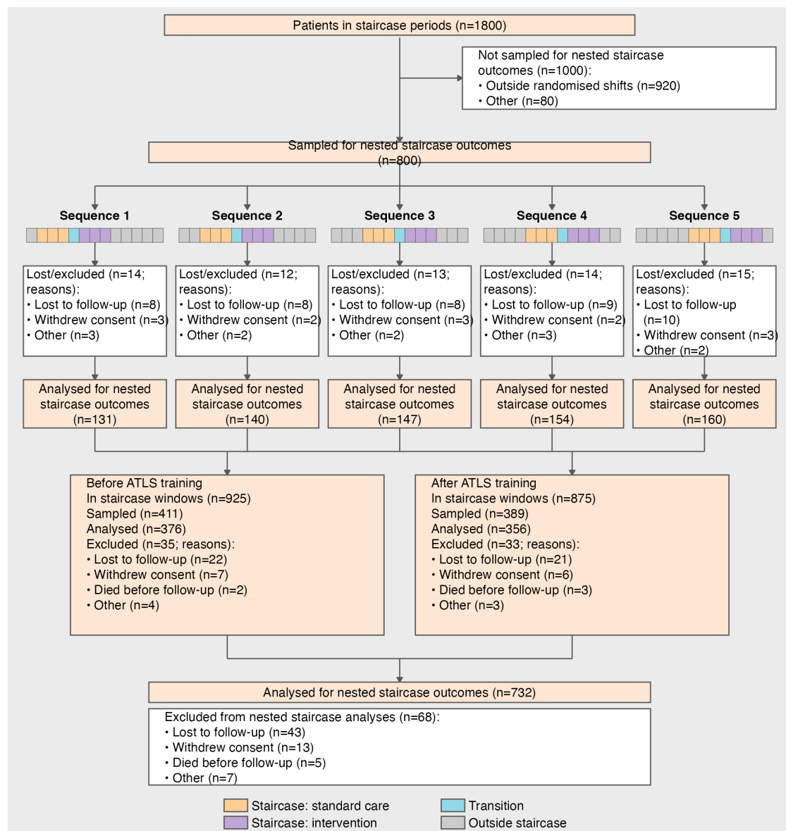
Figure 7: Nested-staircase CONSORT diagram shell with simulated counts. Boxes cover patients in staircase periods, the shift-stratified nested sample, losses and exclusions with reasons, and patients analysed for nested-staircase secondary outcomes, by sequence, before and after ATLS training, and overall. Coloured strip cells mark staircase months; grey cells are outside nested data collection. The flowchart summarises data across all batches 1-6. Intended for the supplementary material.
