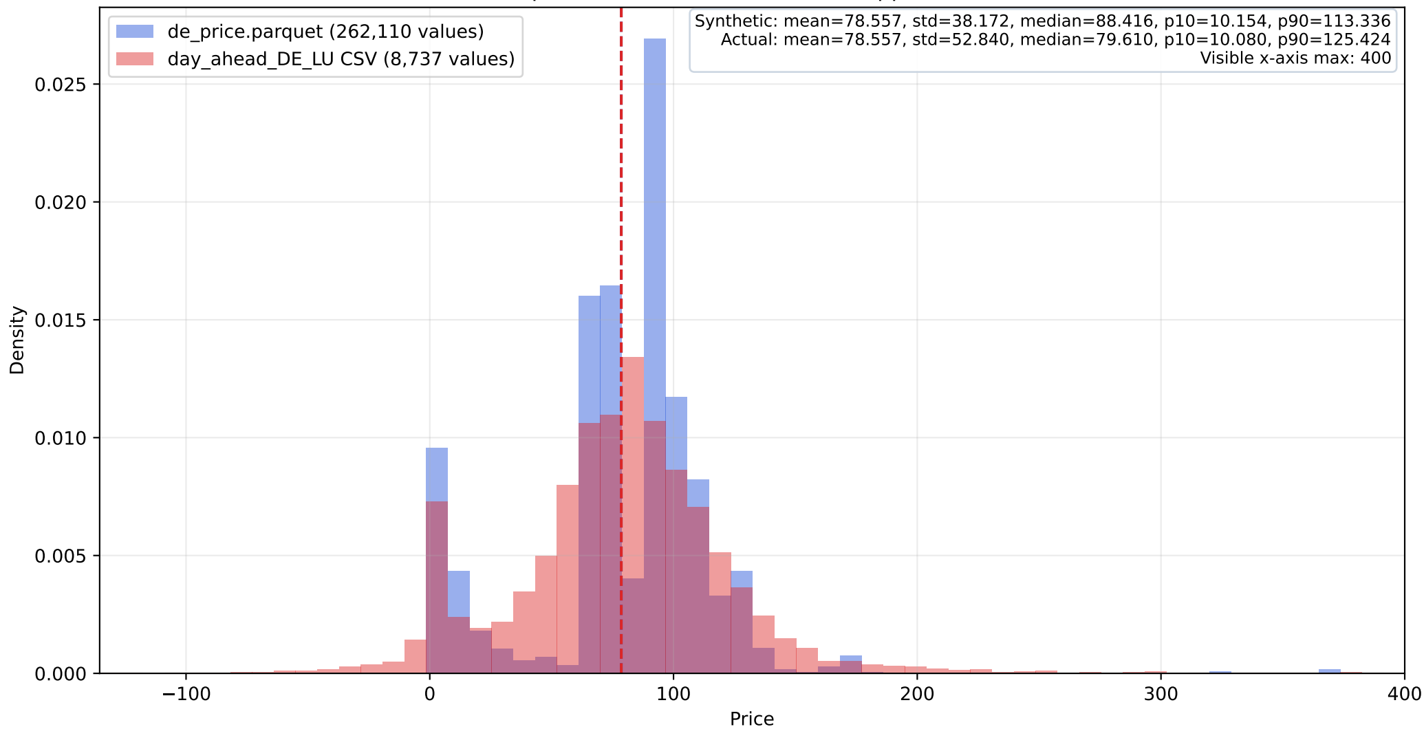
DE price distribution with x-axis capped at 400
