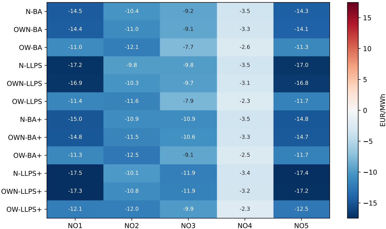
NO Area Mean Price Change from 23 TWh Baseline
