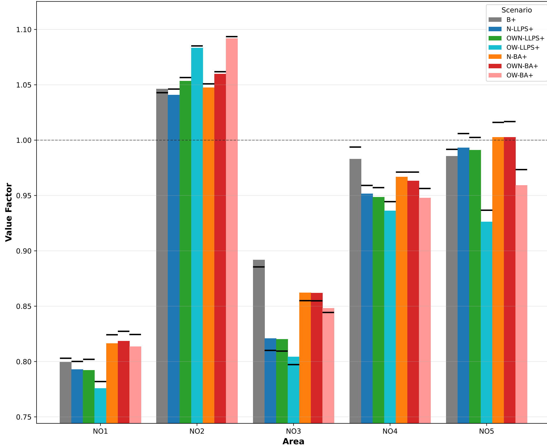
All Hydropower Value Factor by Area
