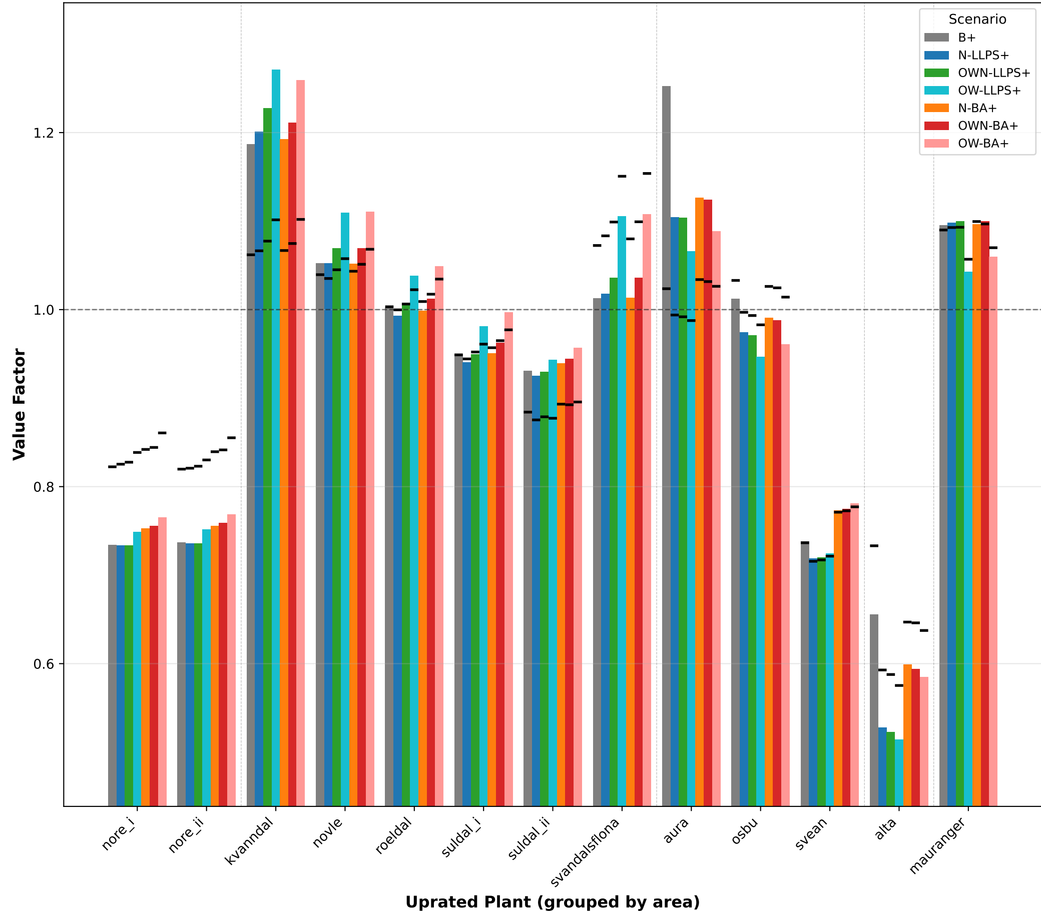
Uprated Plant Value Factor by Scenario
