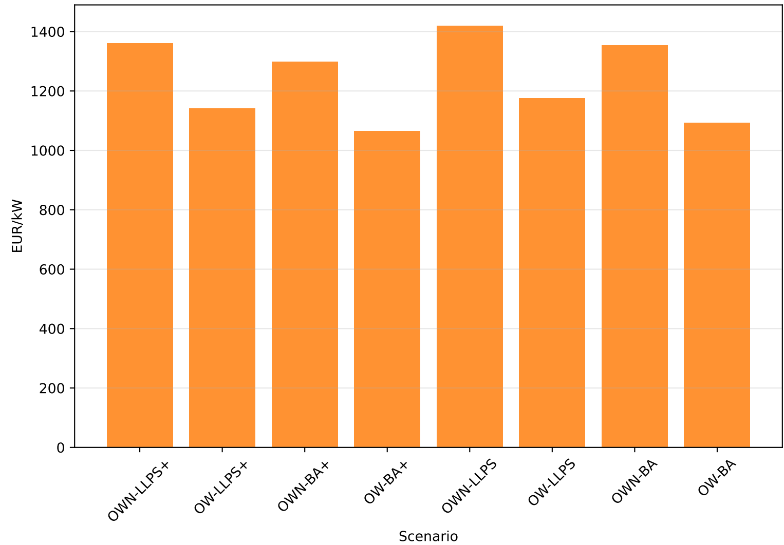
Offshore Wind Inferred CAPEX (FID)
