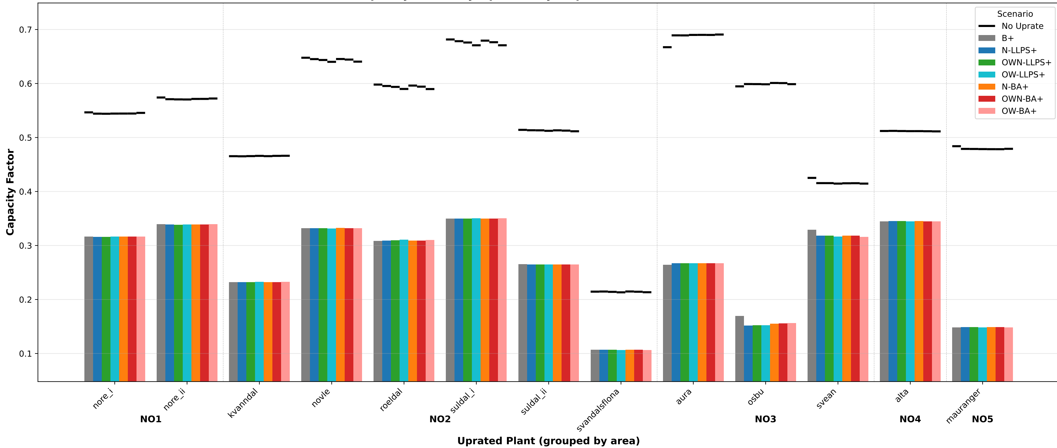
Capacity Factor by Uprated Hydropower Plant and Scenario
