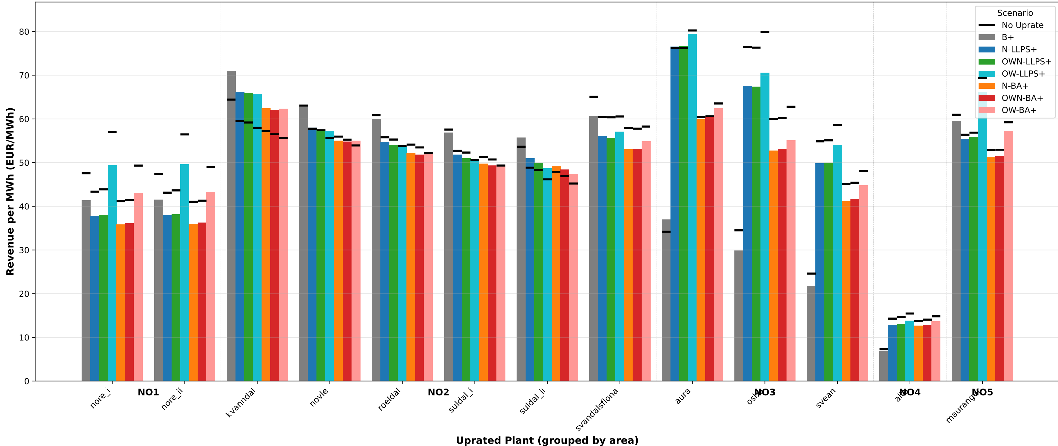
Revenue per MWh by Uprated Hydropower Plant and Scenario
