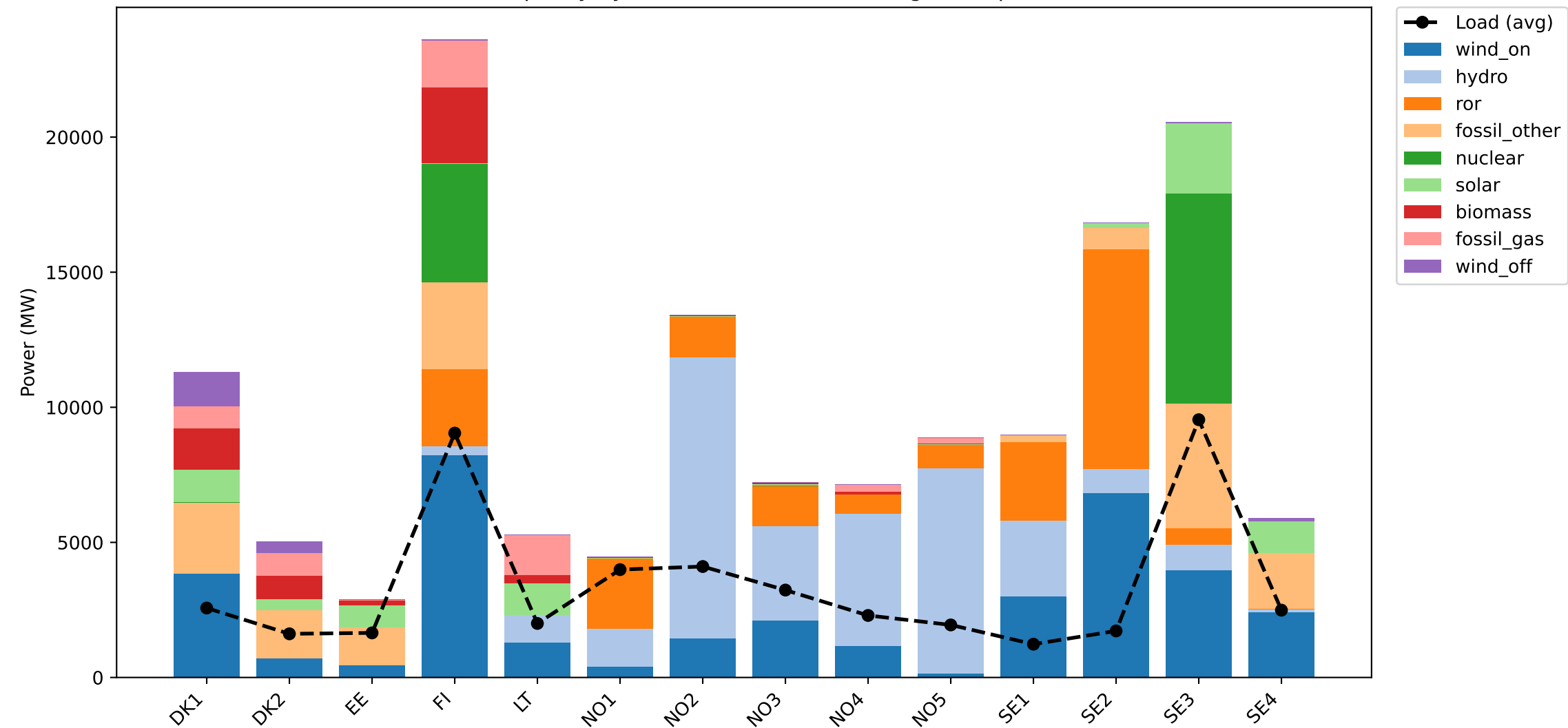
Installed capacity by area (stacked) and average load per area
