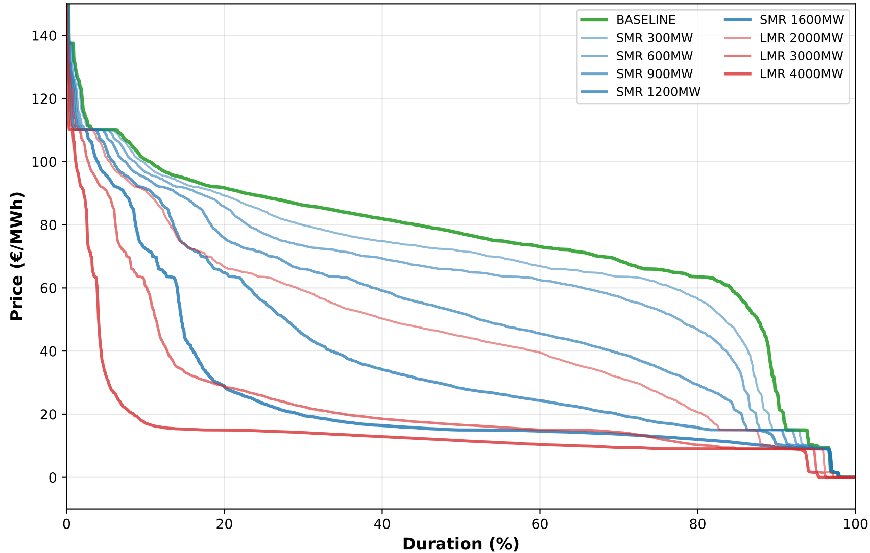
NO2 Price Duration Curve - LLPS Scenarios
