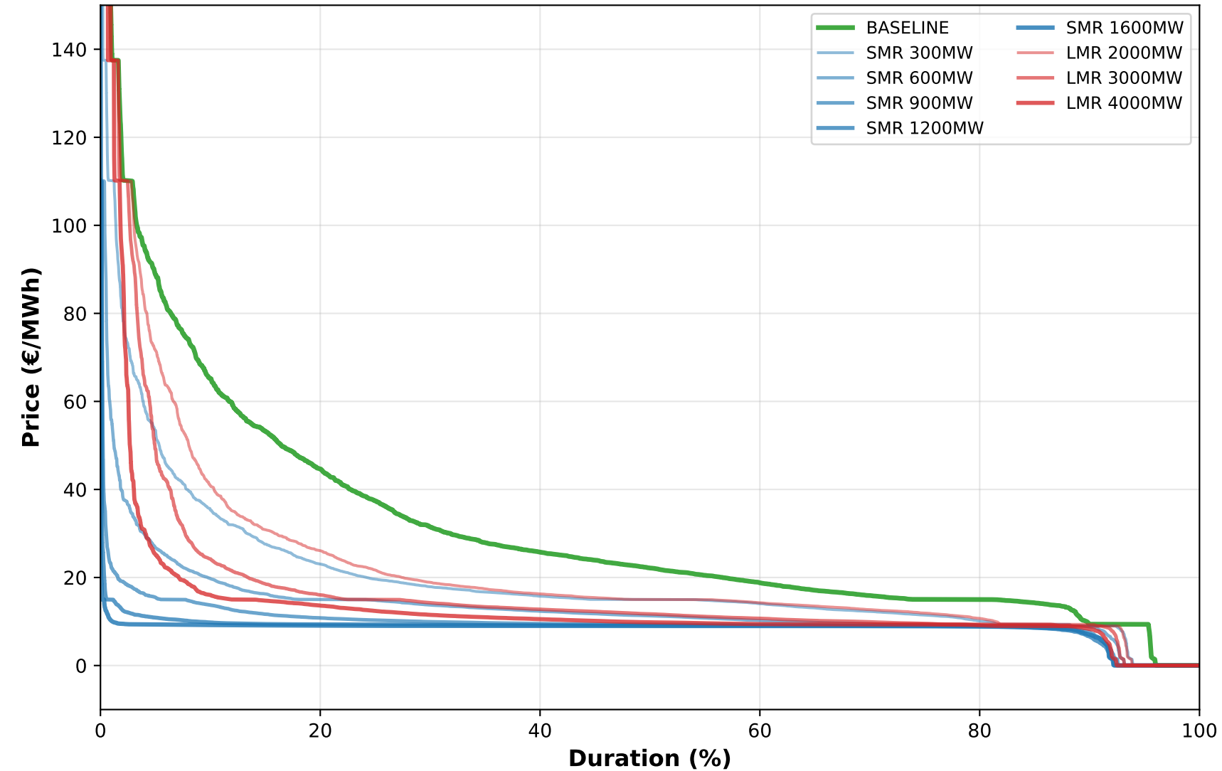
NO4 Price Duration Curve - LLPS Scenarios
