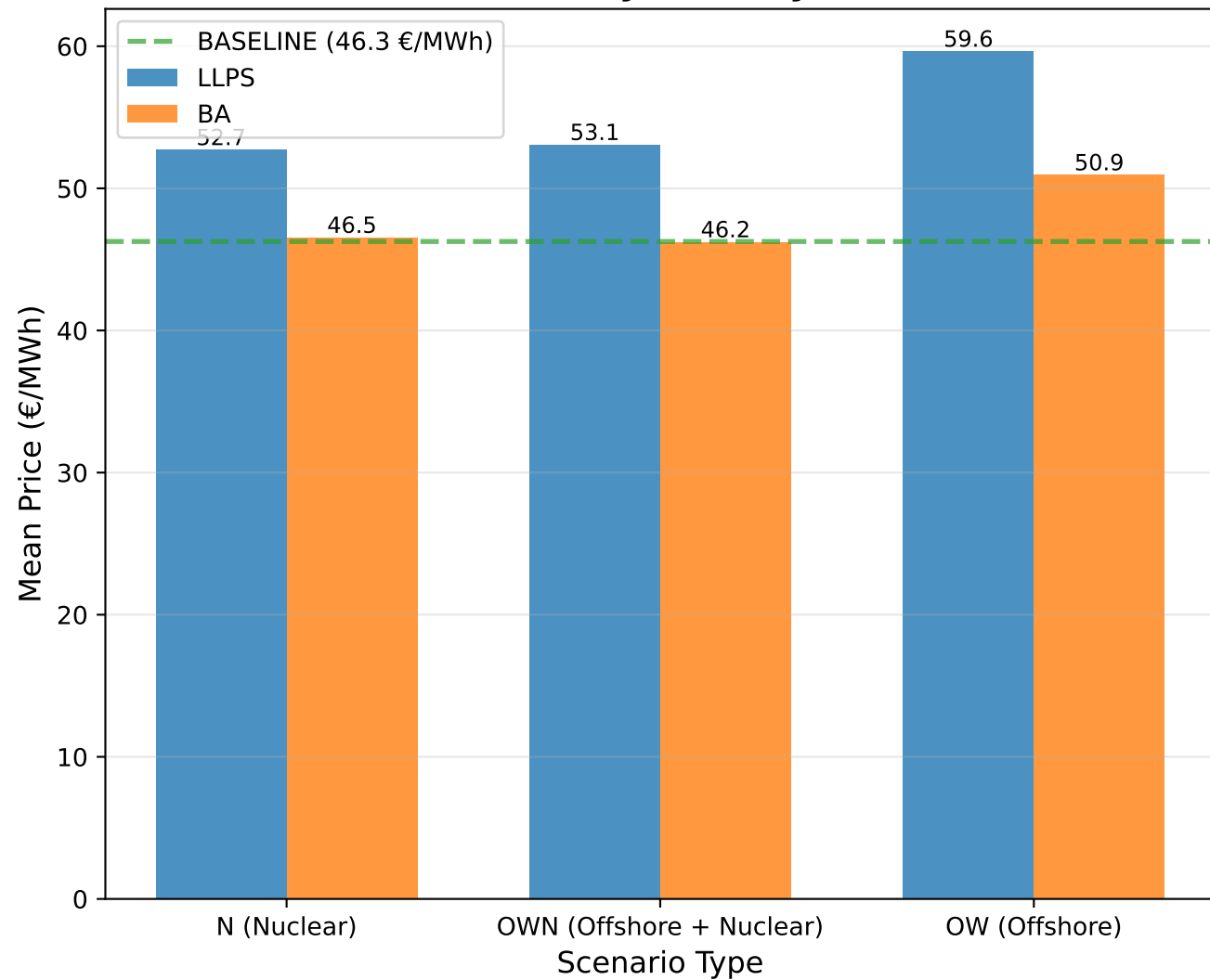
Mean Electricity Price by Scenario
