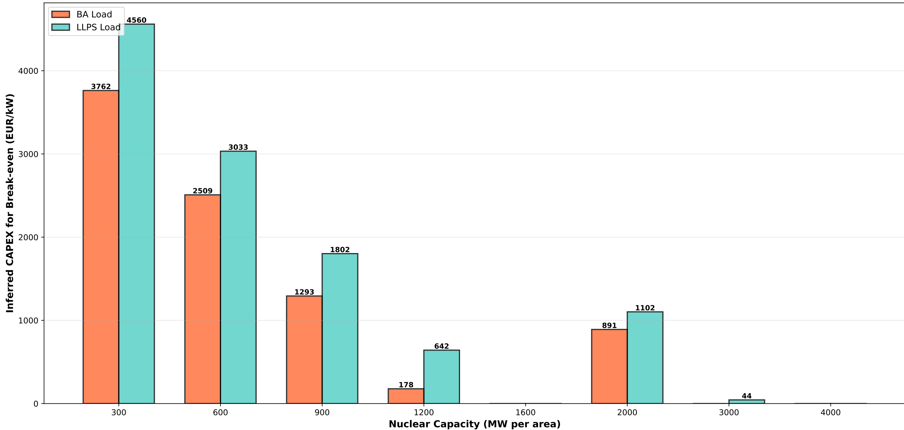
SMR/LMR Inferred CAPEX for Break-even: BA vs LLPS Load Scenarios
