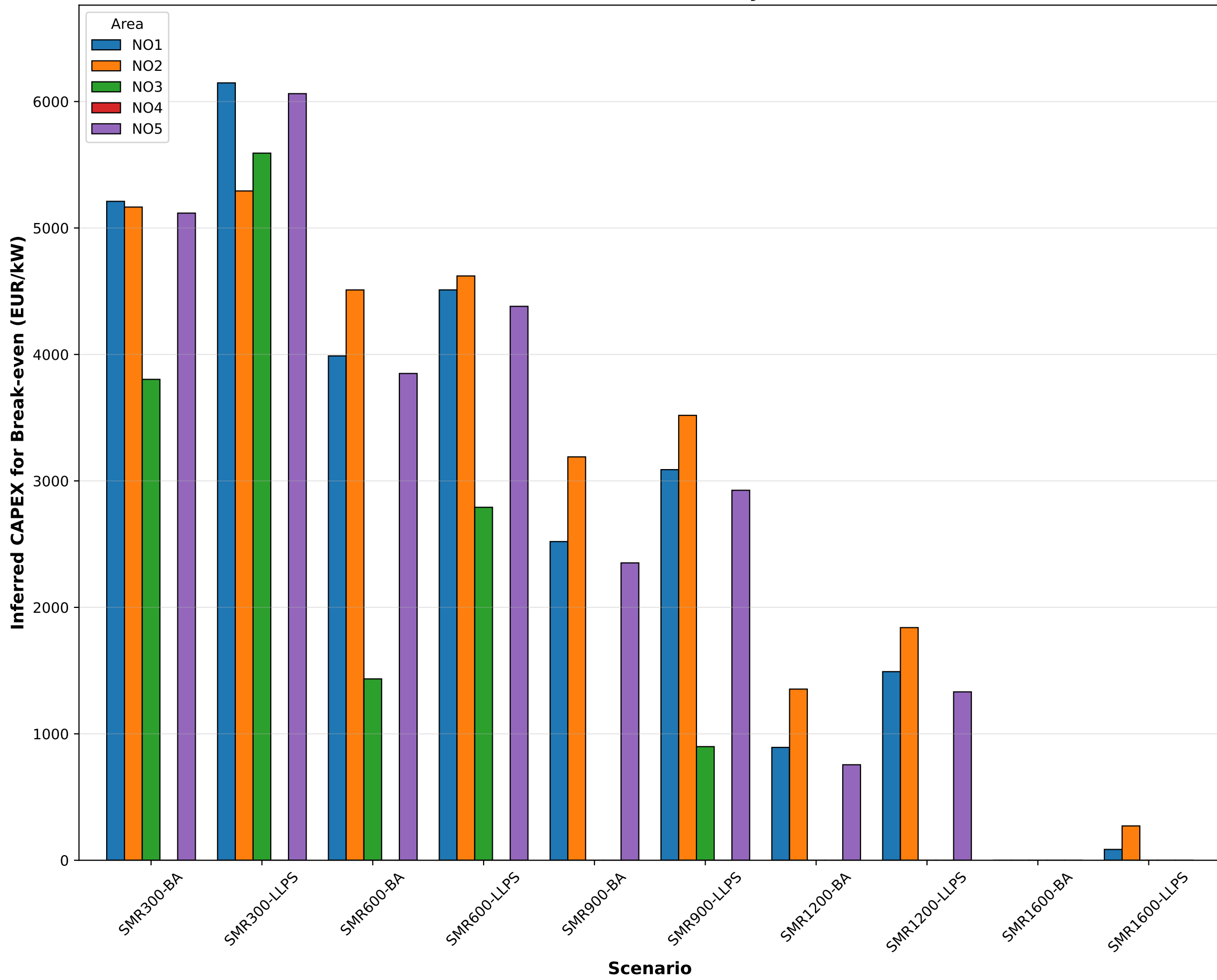
SMR Inferred CAPEX for Break-even by Scenario and Area
