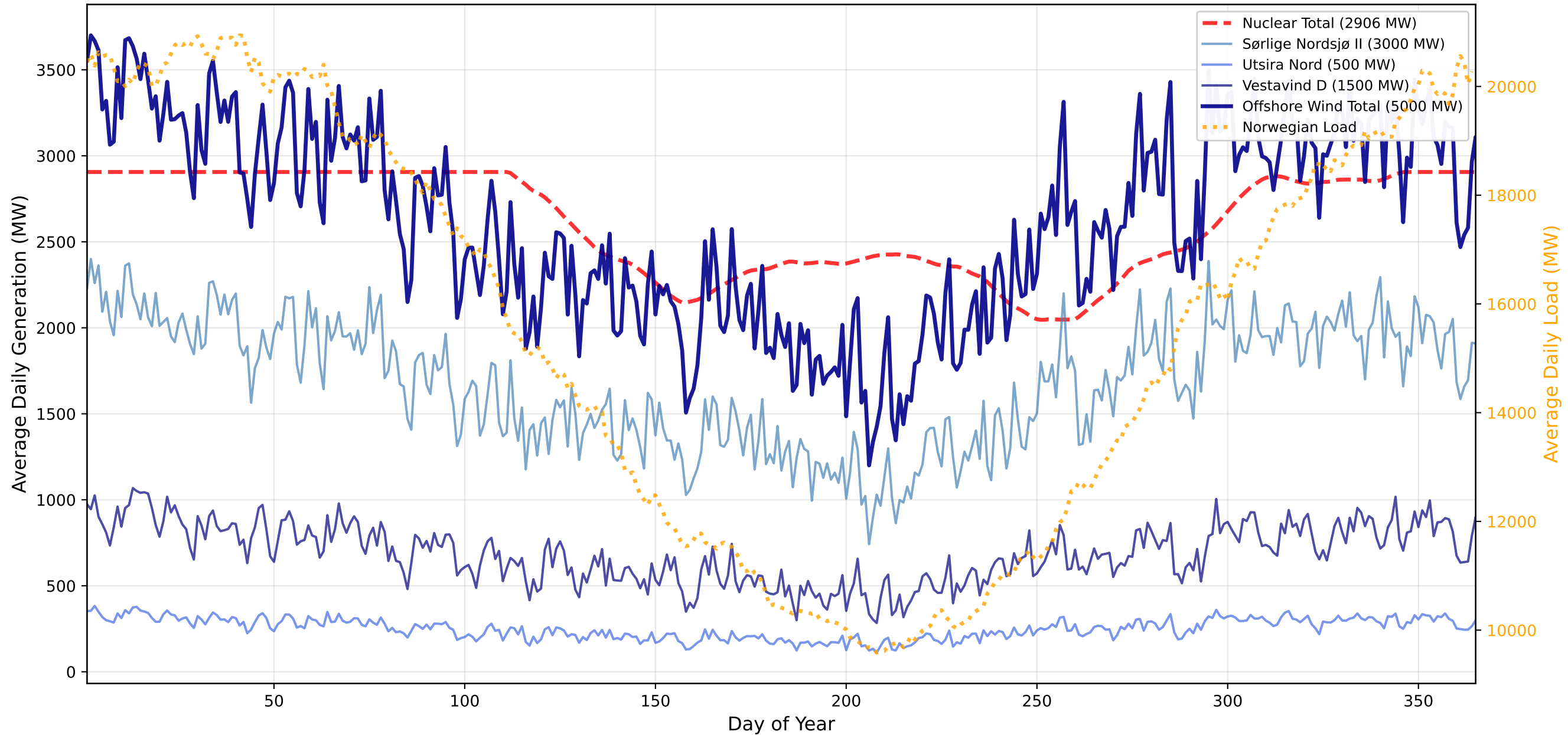
Offshore Wind, Nuclear, and Load Profiles
