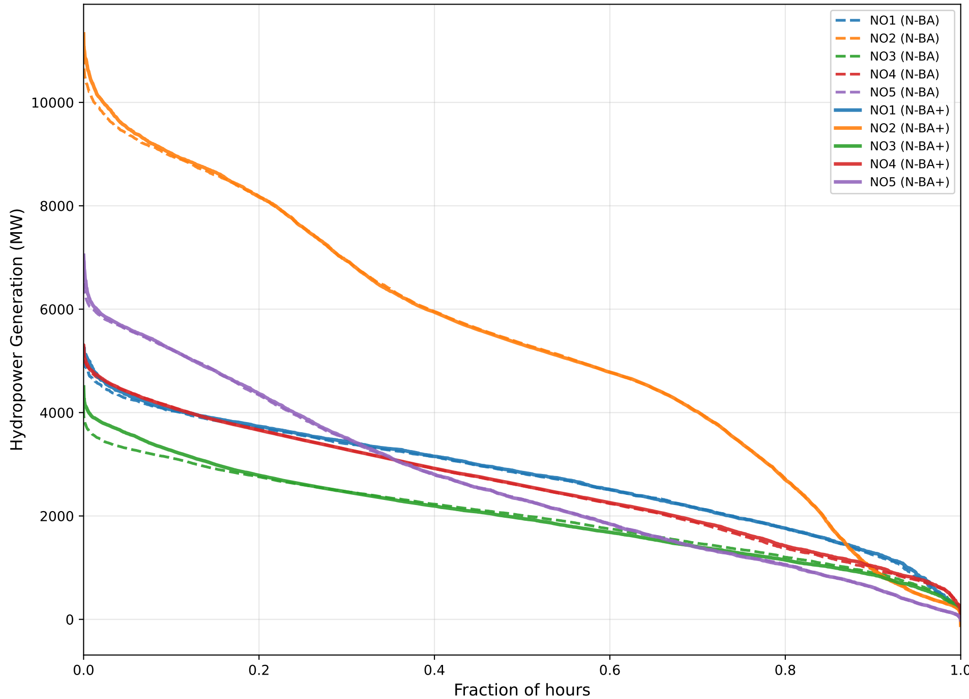
Hydropower Duration
