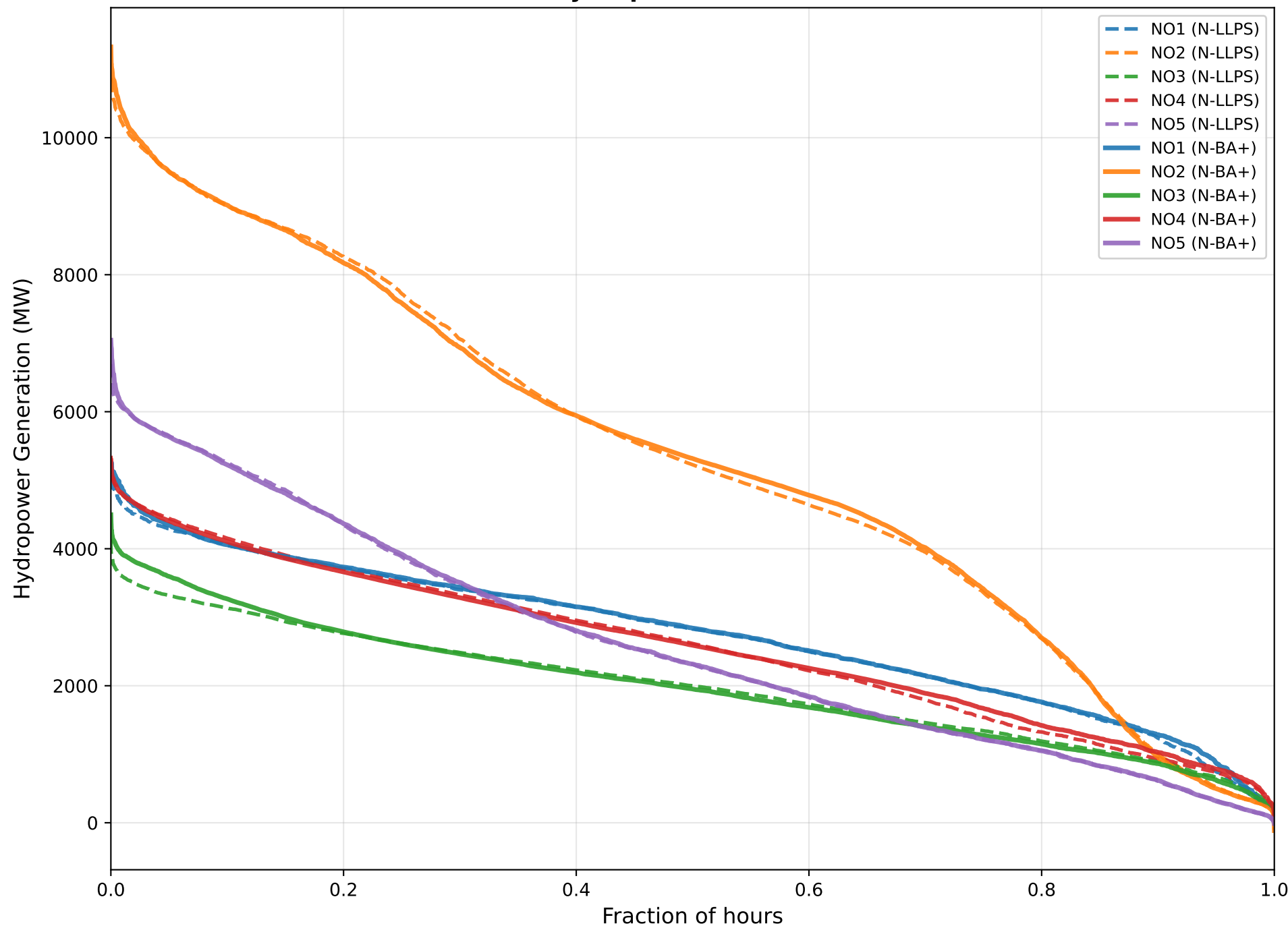
Hydropower Duration
