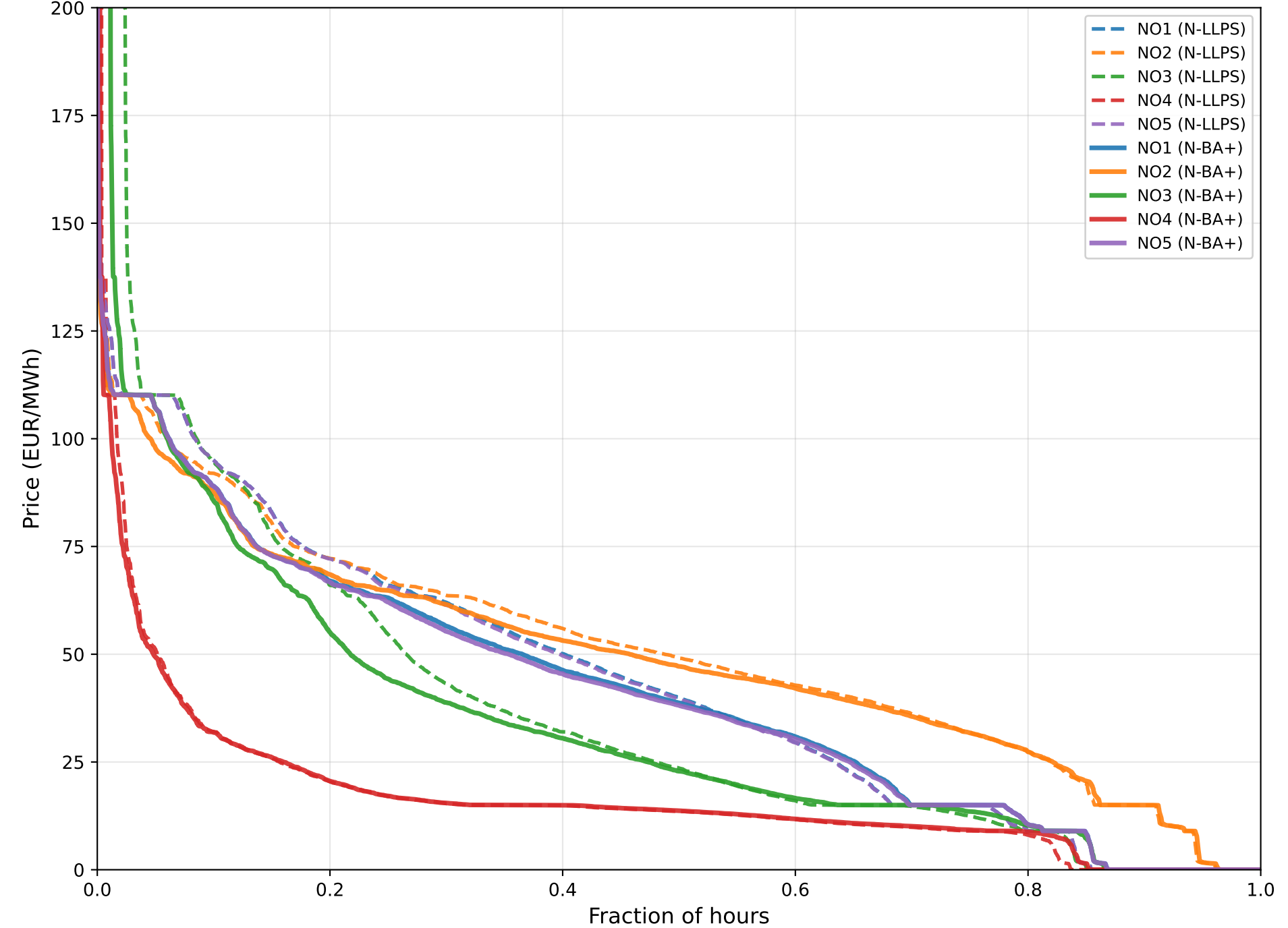
Price Duration
