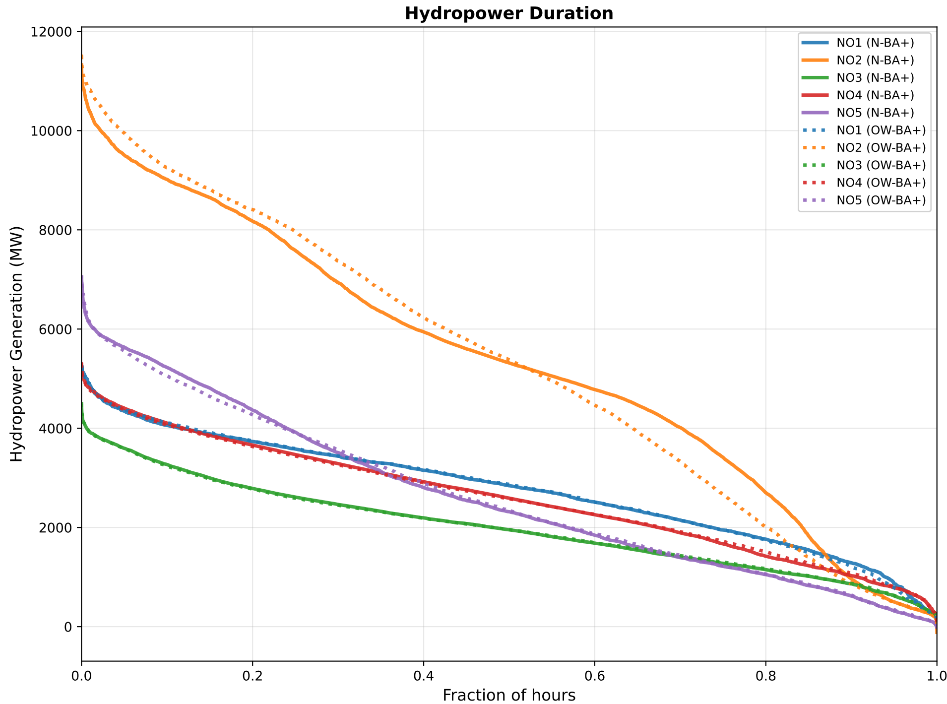
Hydropower and Price Duration Curves - N-BA+ vs OW-BA+ (NO1-NO5)
