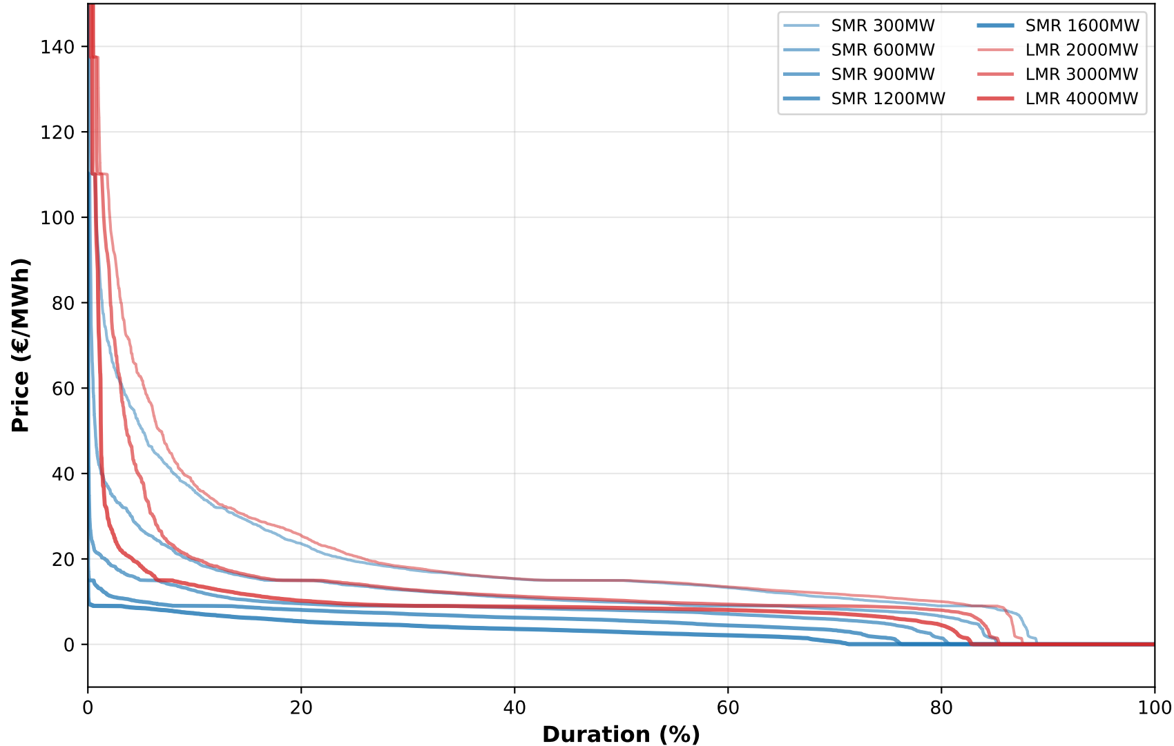
NO4 Price Duration Curve - BA Scenarios
