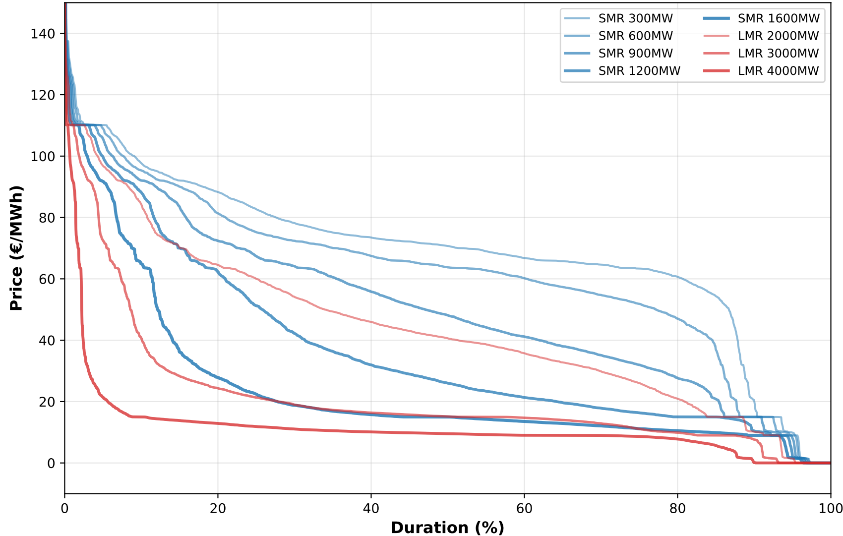
NO2 Price Duration Curve - BA Scenarios
