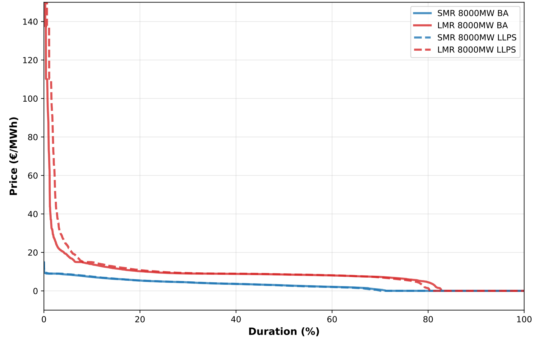
NO4 Price Duration - Maximum Capacity Comparison
