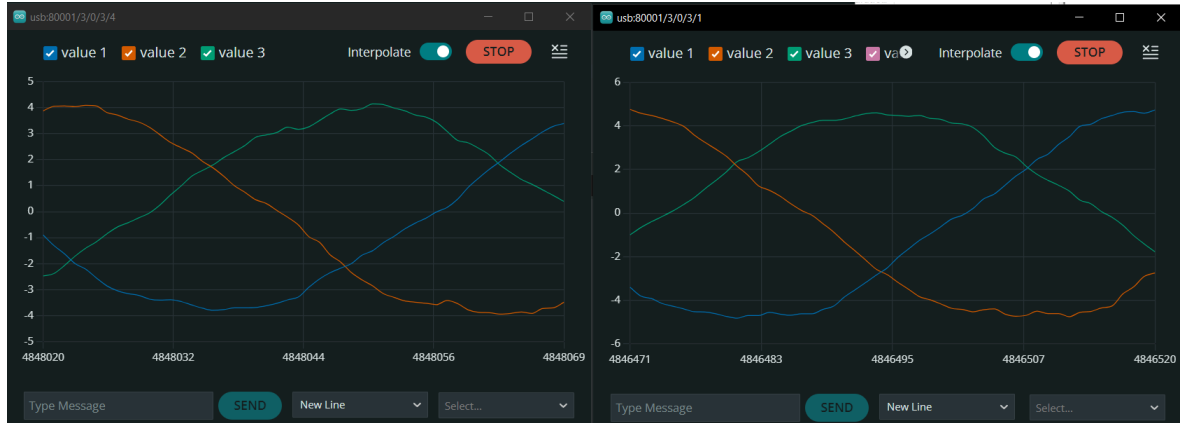
Figure 24: Phase currents from both nodes during synced operation. UART data from the Teensy boards shows both motors spinning at the exact same operator-commanded speed, with classic sinusoidal waveforms from Space Vector PWM under control.
