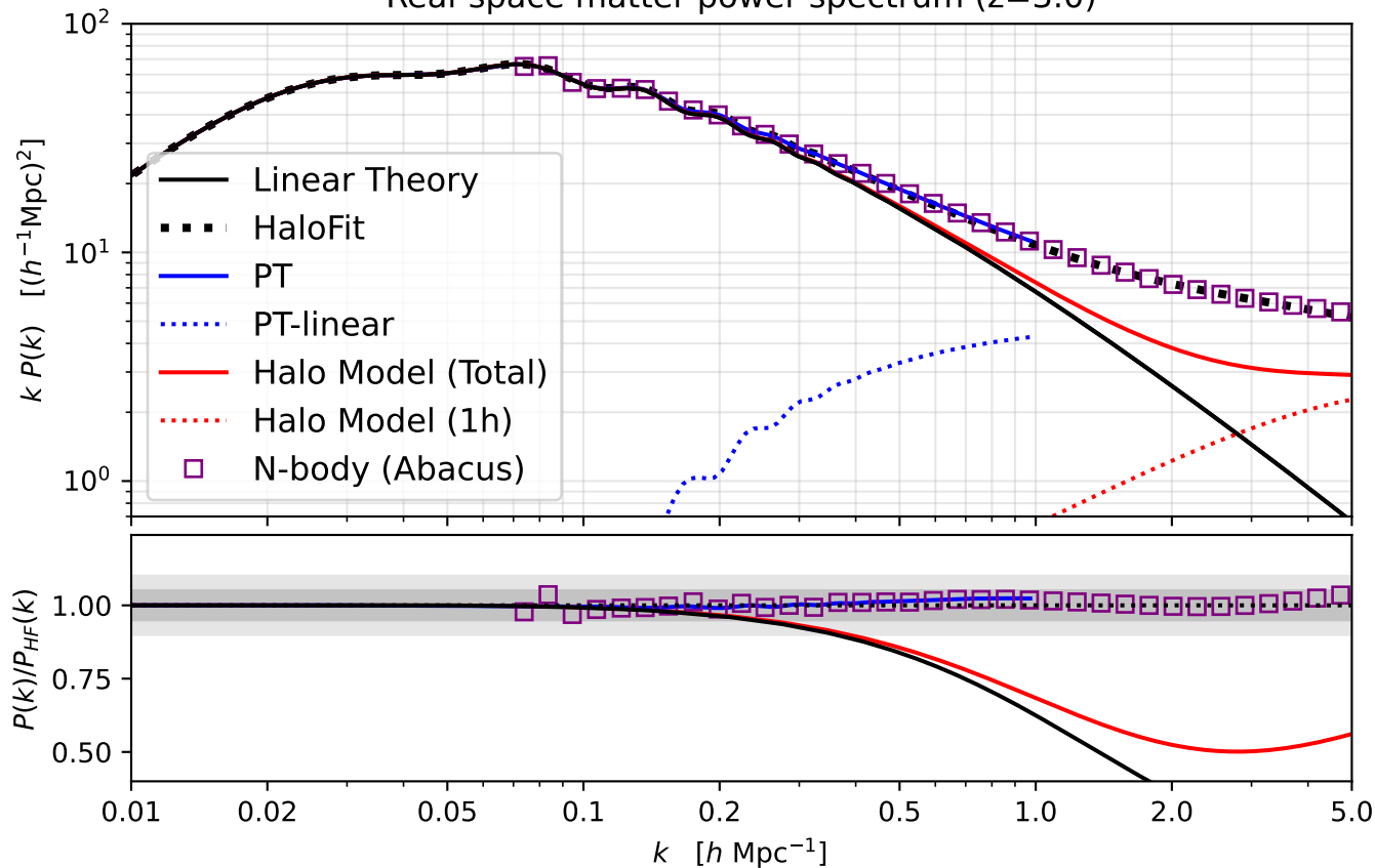
Real-space matter power spectrum ( z=3.0 )
