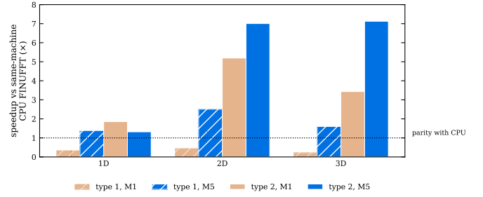
Fig. 4. Cross-machine speedup over same-machine CPU FINUFFT at \varepsilon = 10^{-5} using random points at \rho = 1 . Type-1 spreading is below CPU parity on the M1 and above CPU parity on the M5 Max. Type-2 interpolation is favorable on both systems.
