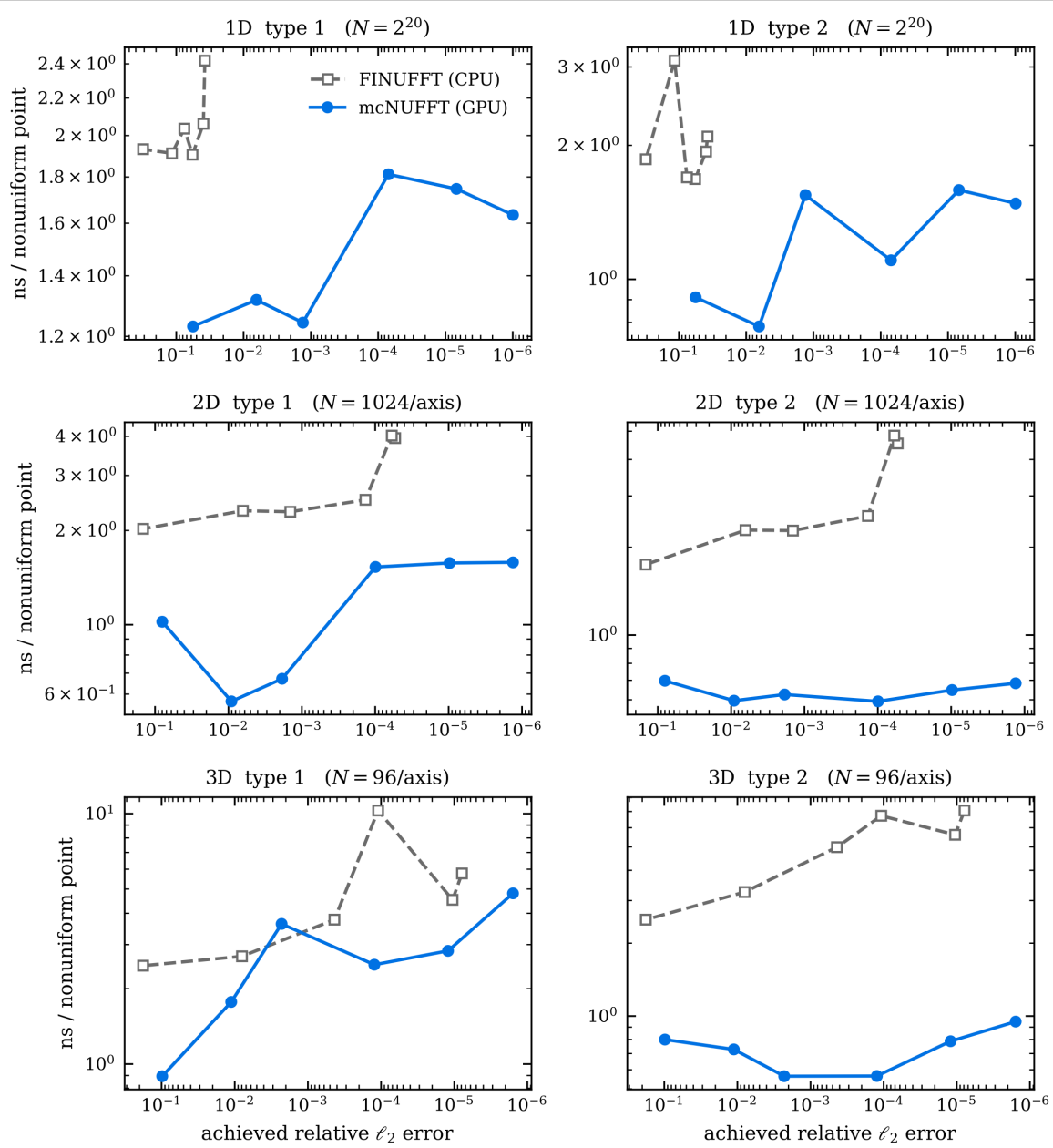
Fig. 1. Signature accuracy and throughput on the M5 Max. The plot shows ns per nonuniform point versus achieved relative \ell_2 error for types 1 and 2 in 1D, 2D, and 3D. The benchmark compares the Metal implementation with same-machine FINUFFT using random points at \rho = 1 . Accuracy increases to the right. In 1D, the single-precision CPU curve stalls near 4 \times 10^{-2} while the Metal implementation reaches 10^{-6} , illustrating the crit64 effect. Non-monotonicity along a curve comes from the integer kernel-width steps and from run-to-run timing scatter at these short per-call times.
