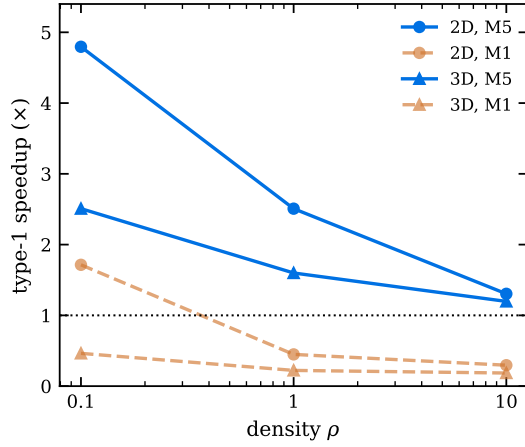
Fig. 3. Type-1 speedup as a function of density \rho . Speedup improves as \rho decreases, especially on the M5 Max, since sparse point sets reduce update contention and make the GPU path more favorable.
