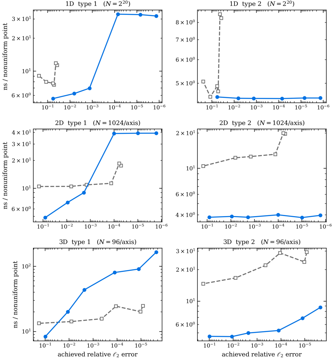
Fig. 2. Signature accuracy and throughput on the M1. Type-2 transforms are faster than same-machine CPU FINUFFT in the tested cases, while type-1 spreading is below CPU parity on this bandwidth-limited system. Compare with the M5 Max results in Fig. 1.
